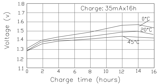
Standard charge
