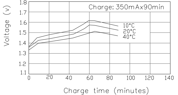
Rapid charge
