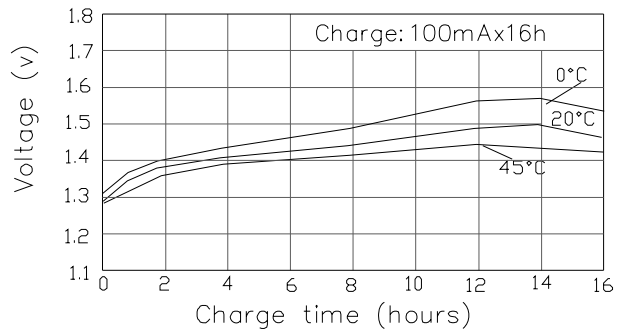
Standard charge
