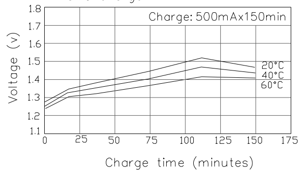
Trickle charge
