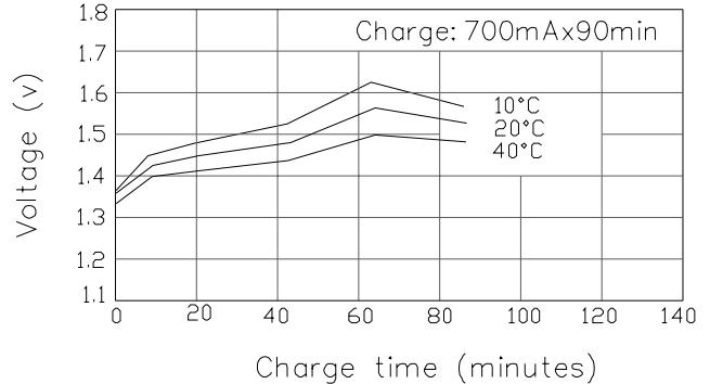
Rapid charge
