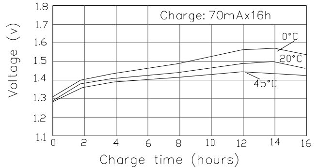
Standard charge
