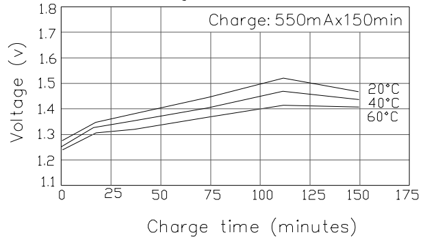
Trickle charge
