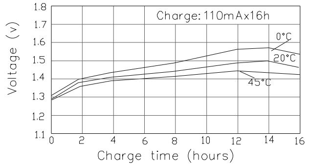
Standard charge
