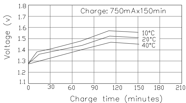
Rapid charge
