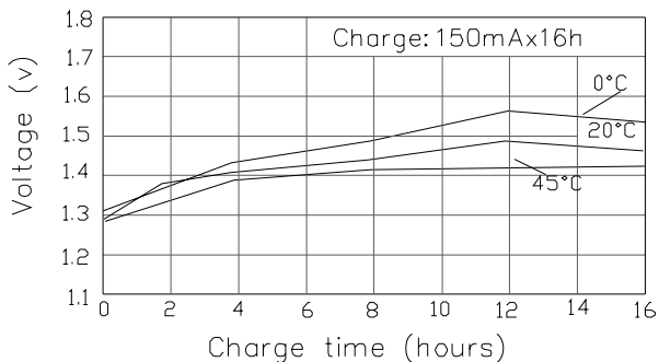
Standard charge
