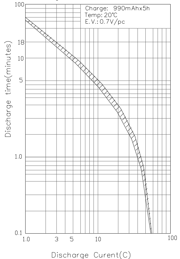
Discharge characteristics
