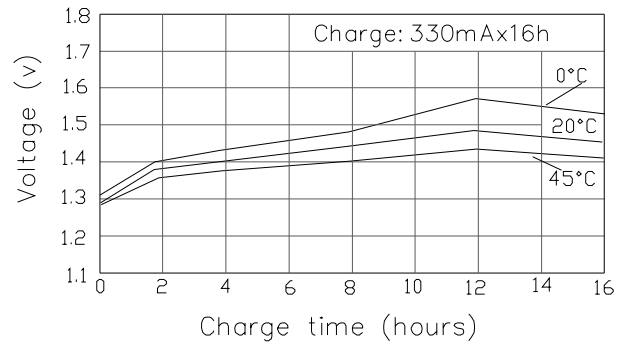
Rapid charge
